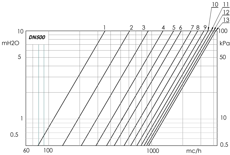
Kv chart (mc/h per bar)
